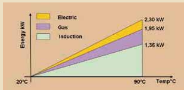
Energy required to heat 12 liters of water from 20° to 90°C
